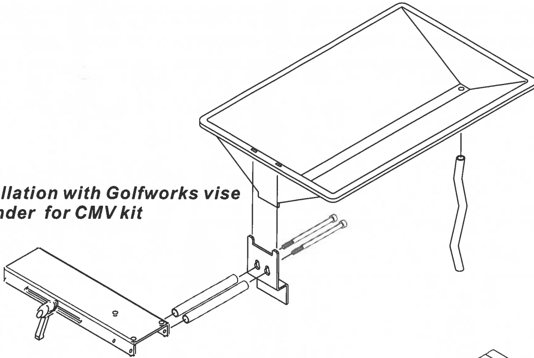
Vise Mount Installation
